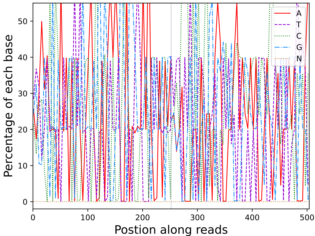
Base percentage along reads (R10520)
